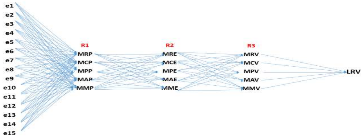
Figure1. Neural networks (Multilayer Perceptron) of the learned meaning of violence
