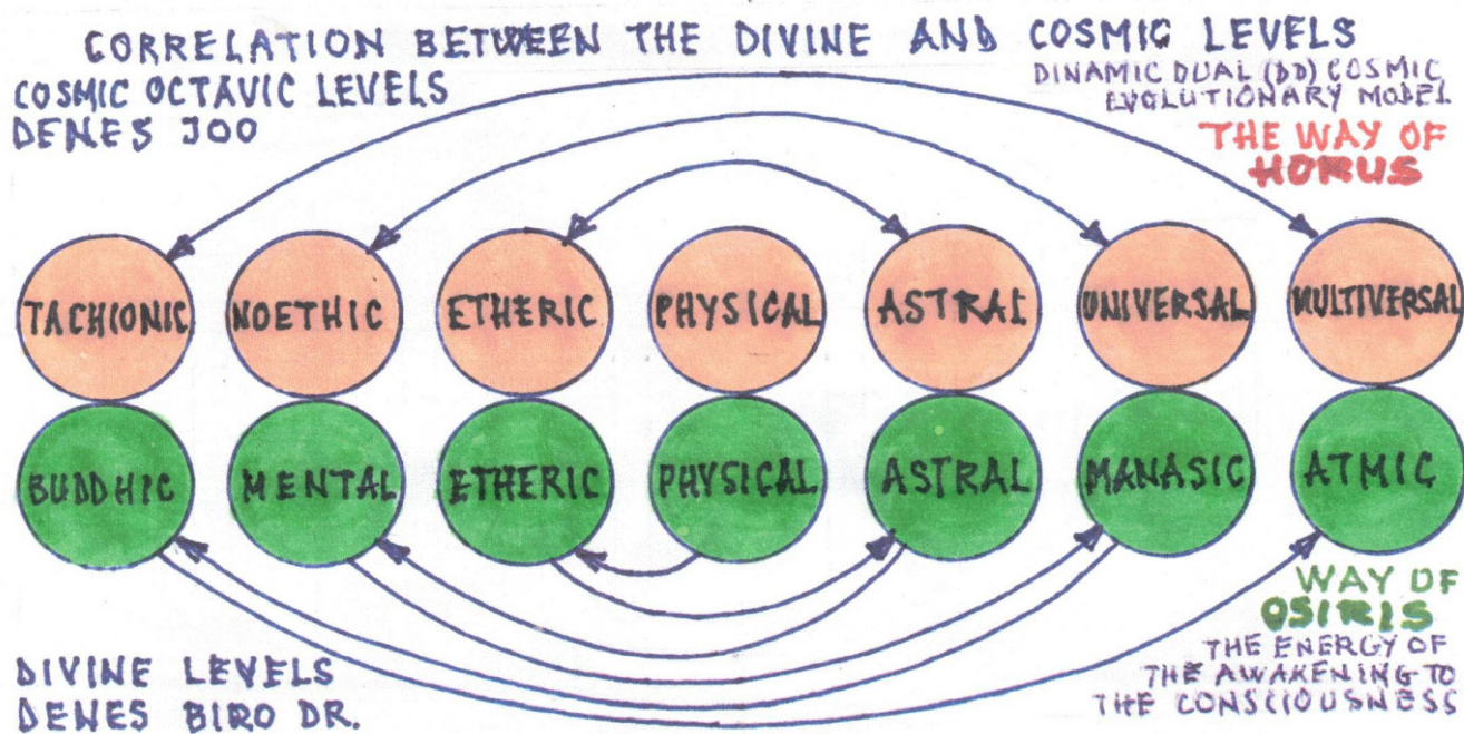
Figure (14). Menora-like Chaotic/Gravitational Connections
