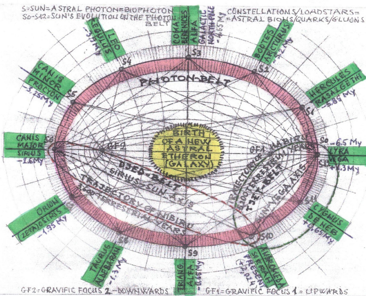
Figure (7). Detailing of the Physical and Astral Cosmic Levels
