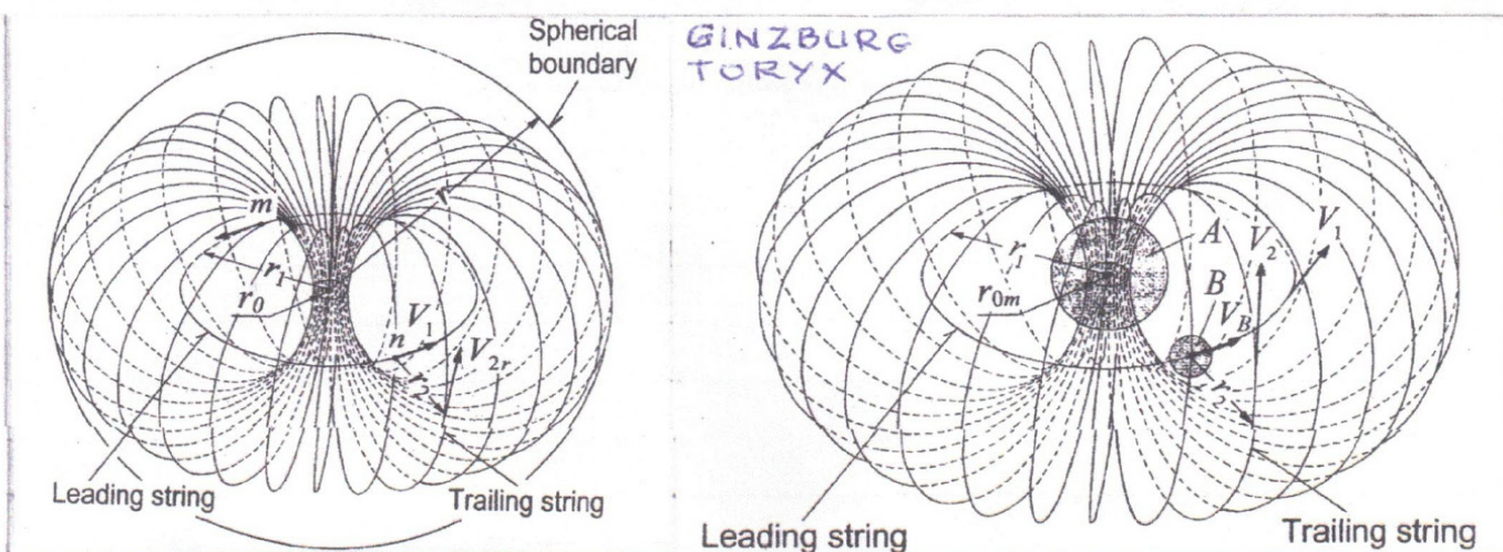
Figure (9). Conic-toroidal Cosmic Evolutionary Model
