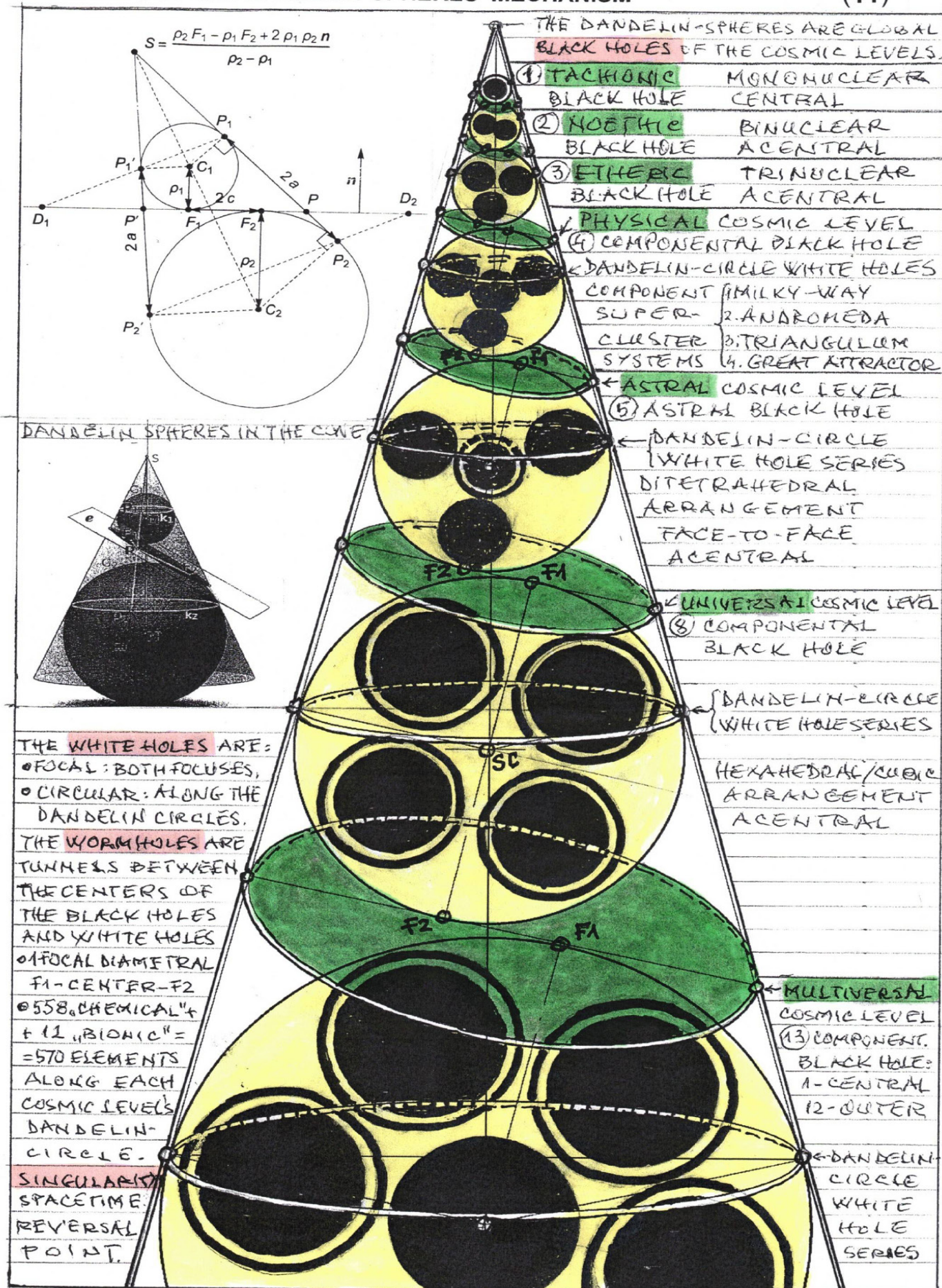
Figure (11). Detailing of the Dandelin-spheres' Mechanism
