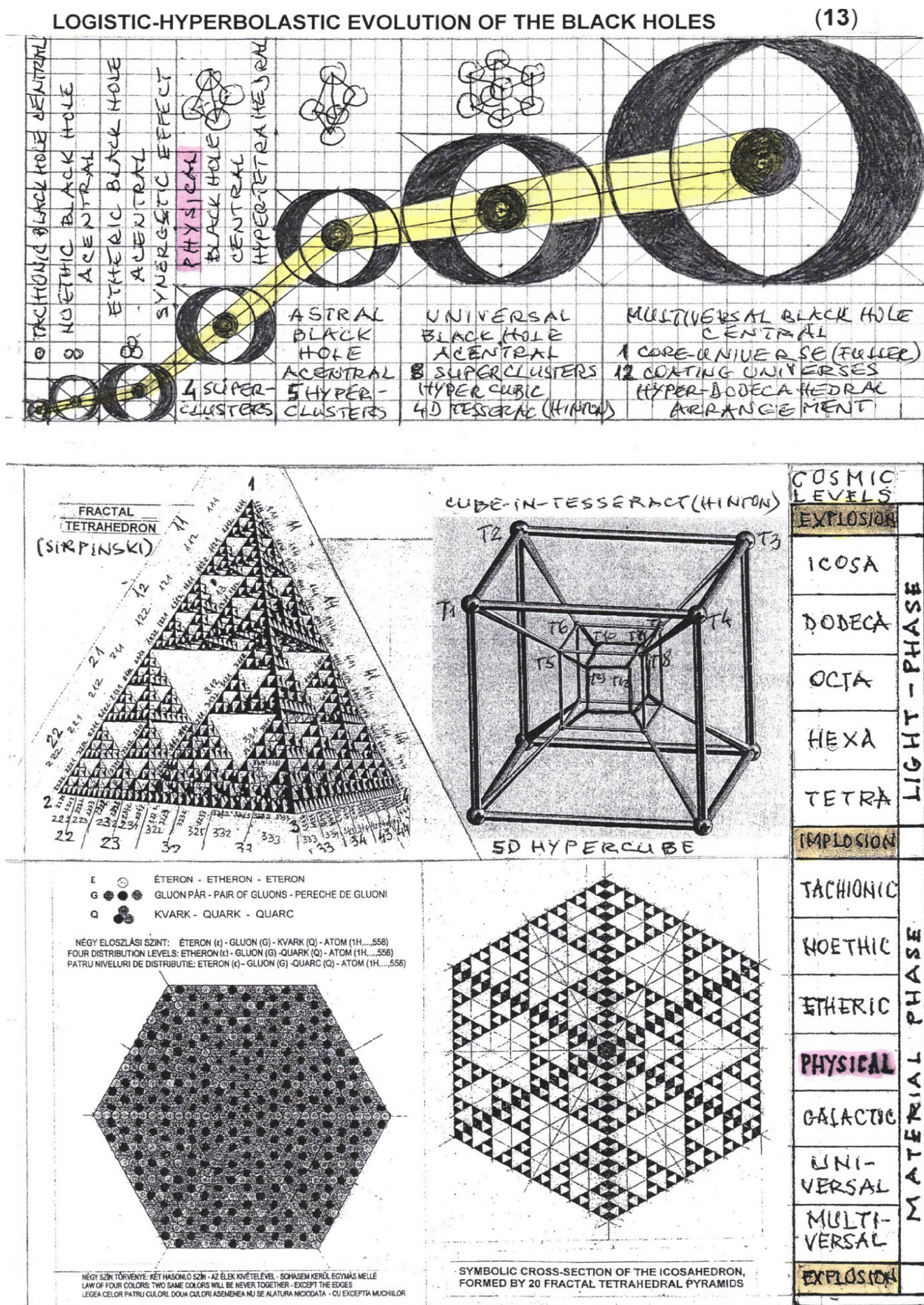
Figure (13). Logistic-hyperbolastic Evolution of the Black Holes
