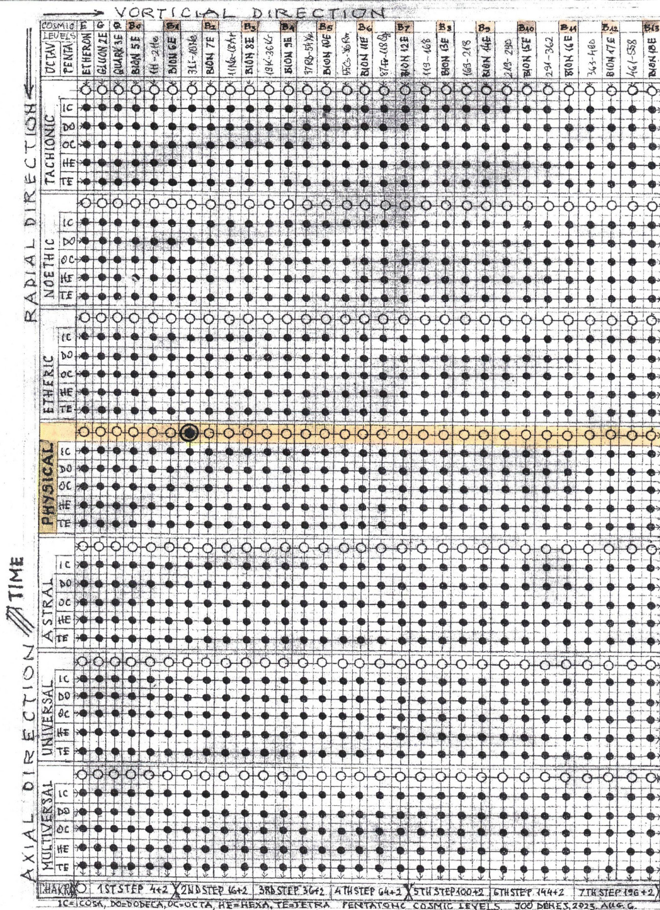
Figure (6). Matricial Quaternionic Cosmic Evolutionary Model
