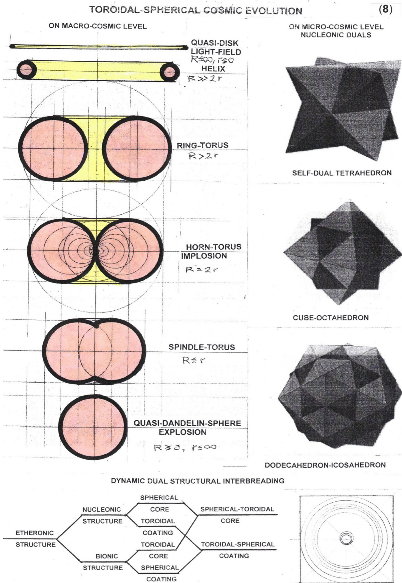
Figure (8). Toroidal-spherical Cosmic Evolution
