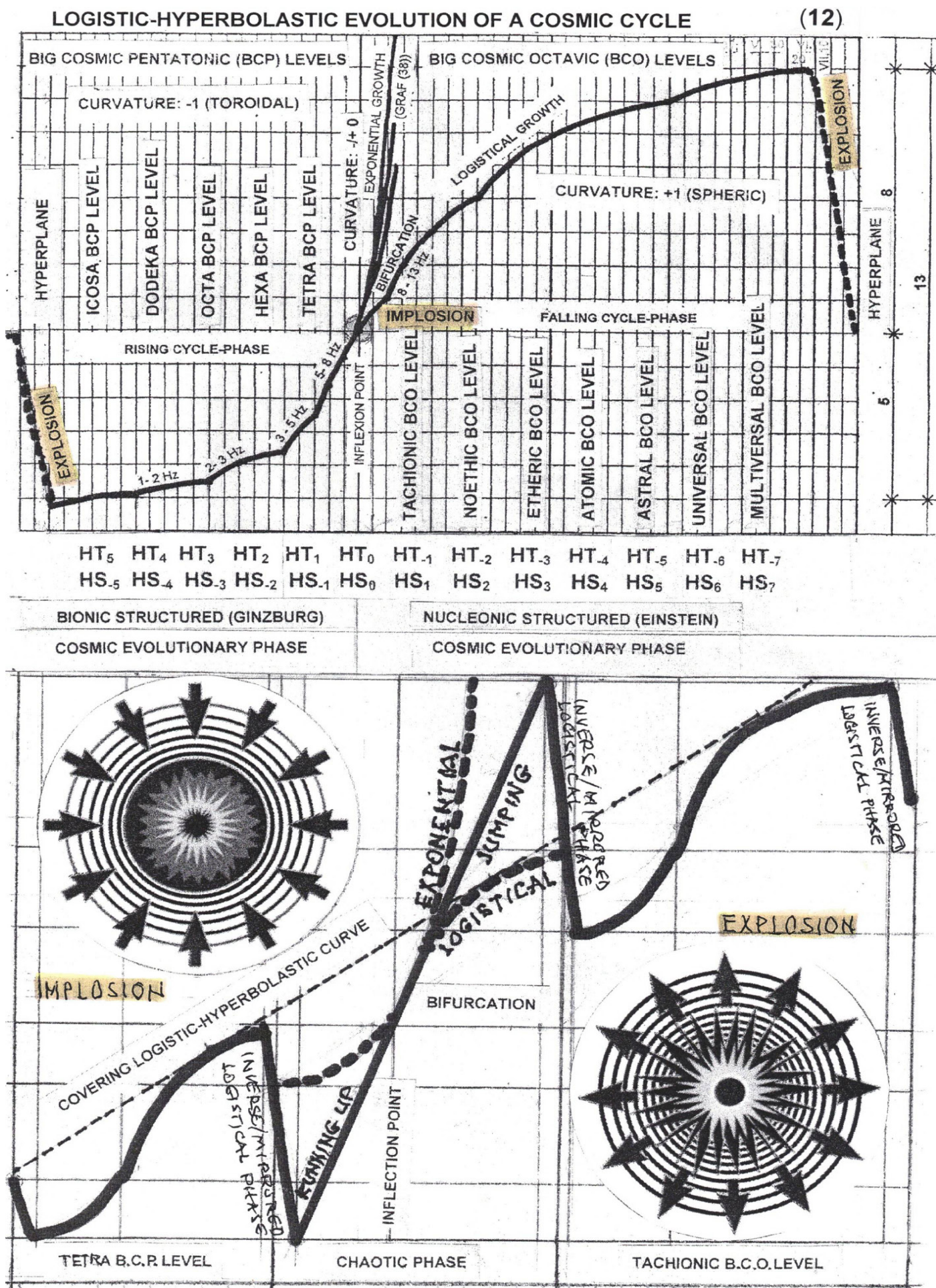
Figure (12). Logistic-hyperbolic Evolution of a Cosmic Cycle
