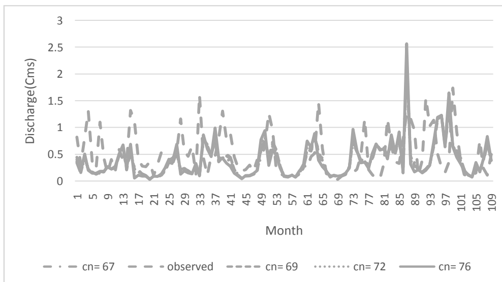
Figure9. River discharge average from different curve numbers as compared with the observed discharge
