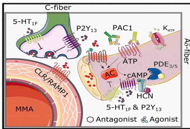
Fig 2. Mechanism of Action
