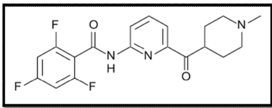
Fig 1. Molecular structure of Lasmiditan
