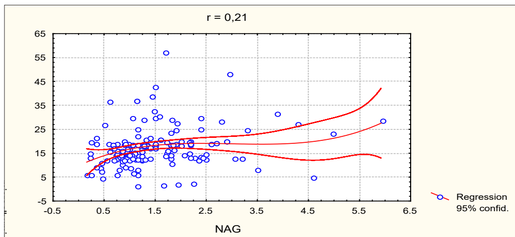
Fig1. Pearson coefficient of correlation ( r ) between NAG and microalbuminuria values in the groups treated with Etoricoxib. There is correlation between NAG and microalbuminuria ( r = 0.21 ).
