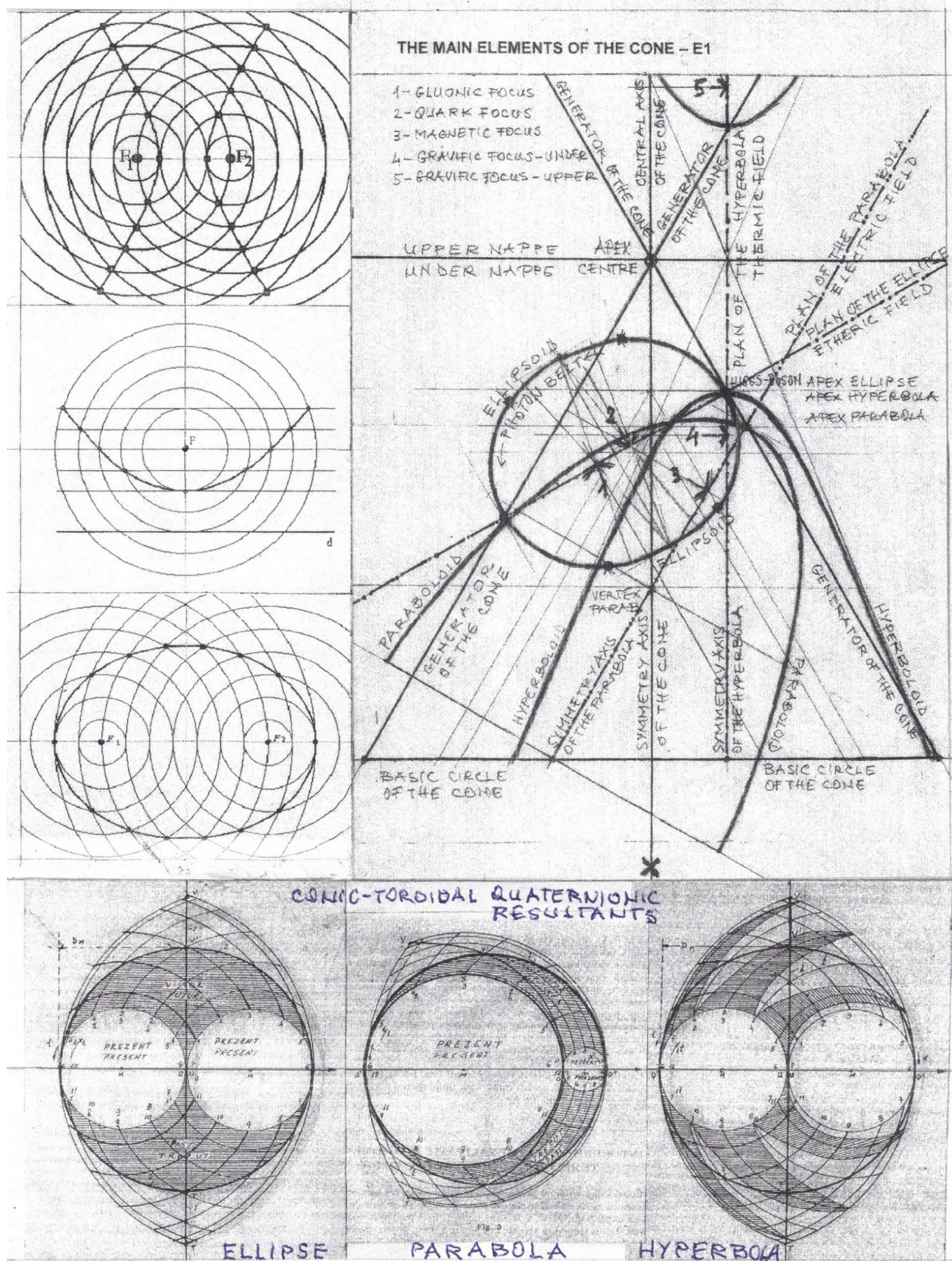
Figure 8. Quaternionic Resultant of the Conic Sections
