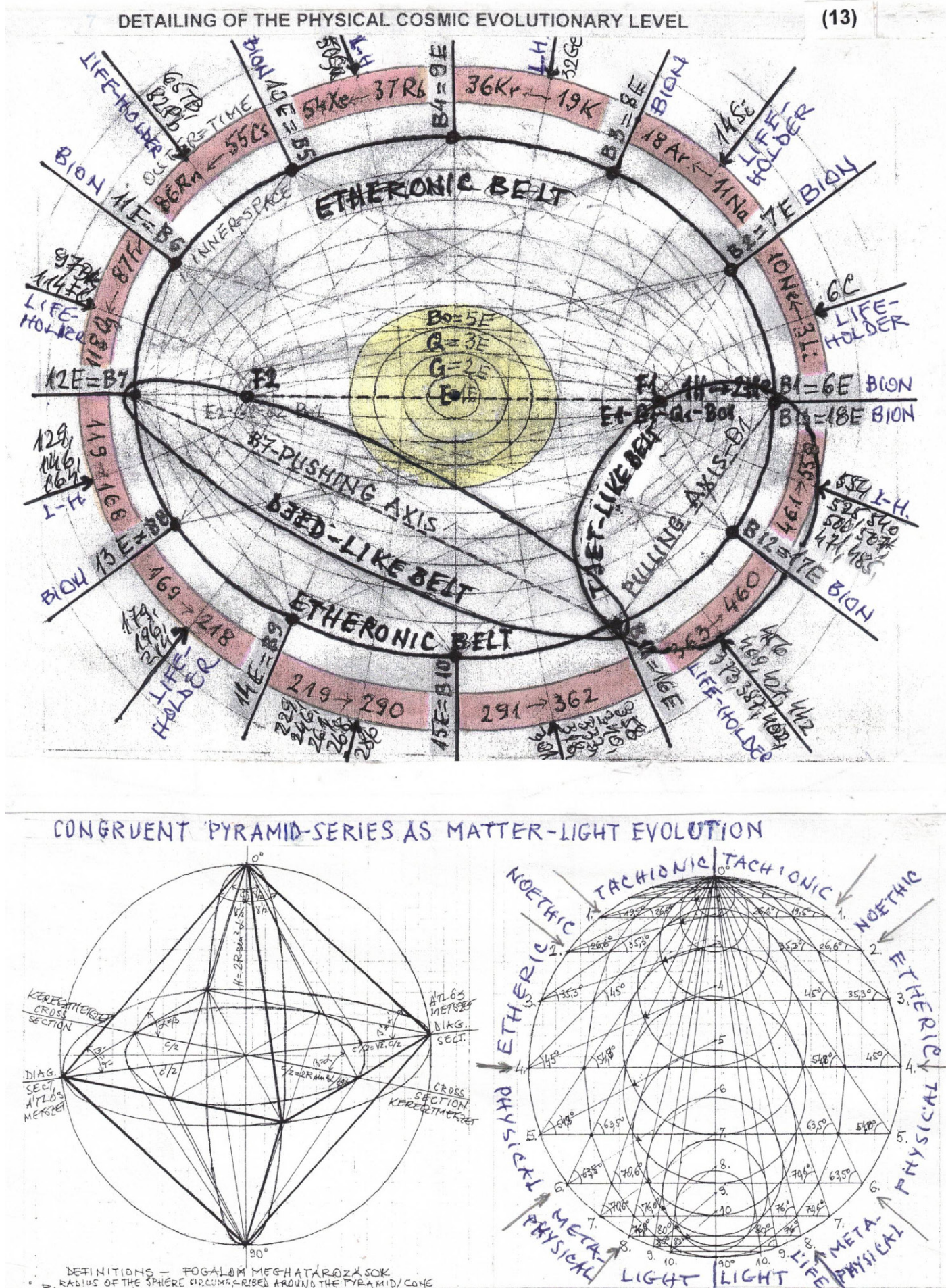
Figure 13. Detailing of the Physical Cosmic Evolutionary Level
