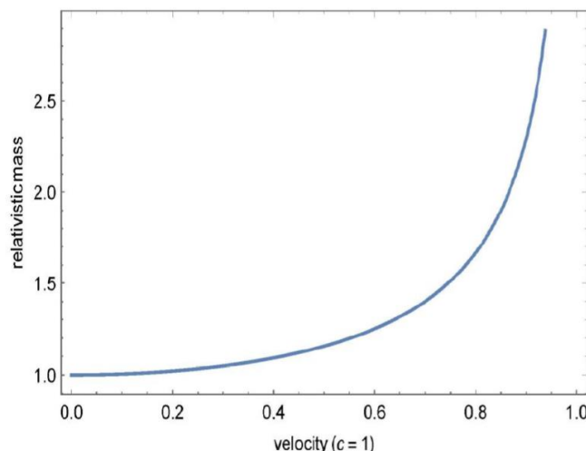
Figure2. Dependency between the mass of a body and its velocity. The graph shows how the mass approaches infinity as velocity approaches the speed of light. Thus, it is not possible for an object with mass to reach the speed of light.
