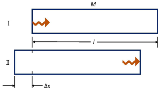
Figure 1. Einstein's box experiment: An isolated box recoils from its initial position (I) to a final position (II) as a result of a photon traveling from one end of the box to the other.
