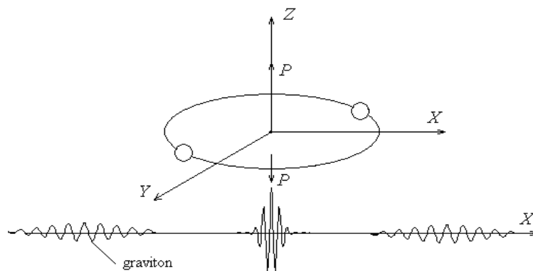
Figure 2. Double star radiating the gravitational waves and a graviton flying in the field of a double star
