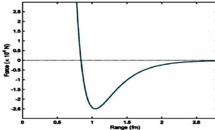
Figure 1. The affecting range of the strong force is very short
