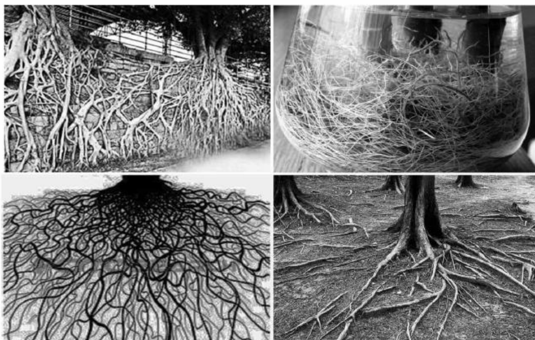
Figure 2. Quark, rhizo-nucleon, its shape is like plants roots by close planting
