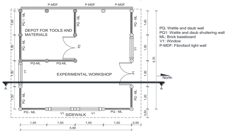
Figure 6. Experimental Workshop floor plan.
