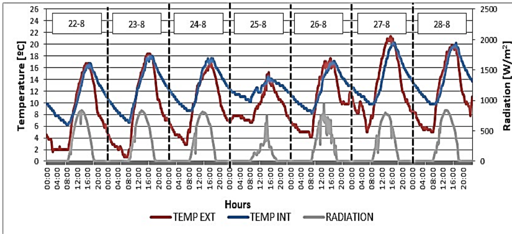
Figure 17. Thermal behavior of the E.W.
