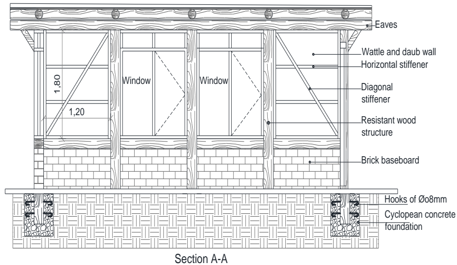
Figure 7. Section plane of Experimental Workshop (E.W.)
