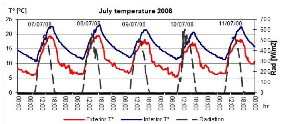
Figure 18. Interior and exterior temperatures of the E.W. (Figure from Cuitiño et al, 2008)
