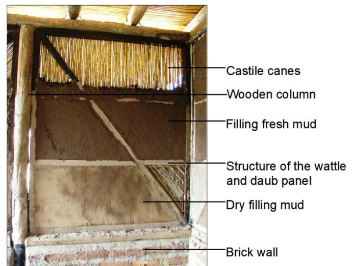
Figure 10. Detail of wattle and daub wall infill techniques
