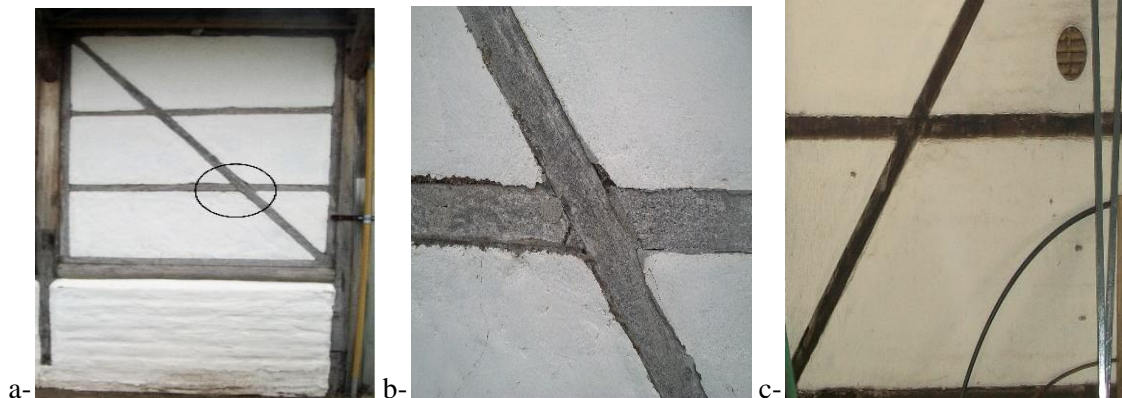
Figure14. Pathologies in joints on wattle and daub walls: a- Northern wall. b-Detail exterior joint c- Detail interior joint.
