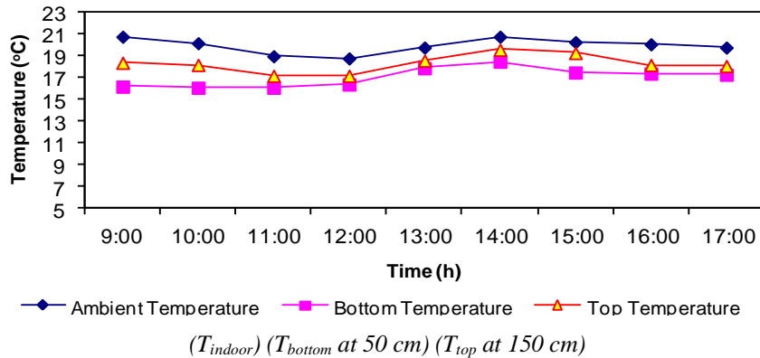
Appendix2.1. Temperature variation in January.
