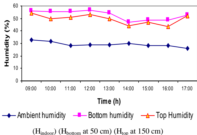
Appendix2.16. Average daily variation of humidity in September
