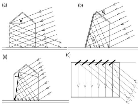
Figure2. Greenhouse types according to the applied mode of reflection of solar radiation: (a) fixed vertical reflecting wall (b) fixed inclined reflecting wall (c) reflecting wall with variable inclination (d) reflecting wall with louvers.
