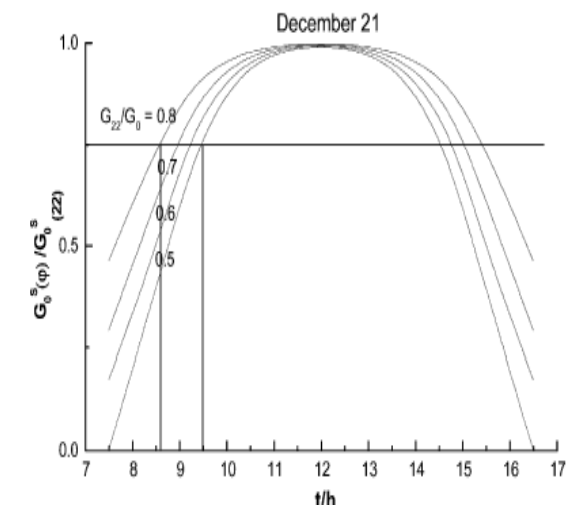
Figure 7. Calculated values of normal irradiance by solar rays relative to the values obtained at the apex on December 21 for different transmittance by the atmosphere.
