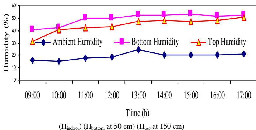
Appendix2.18. Average daily variation of humidity in October
