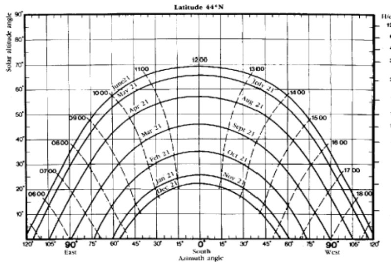
Figure 8. Dependence of the elevation and azimuth angle of the sun on the time of a day at different days of a year at NL 44^\circ [35]
