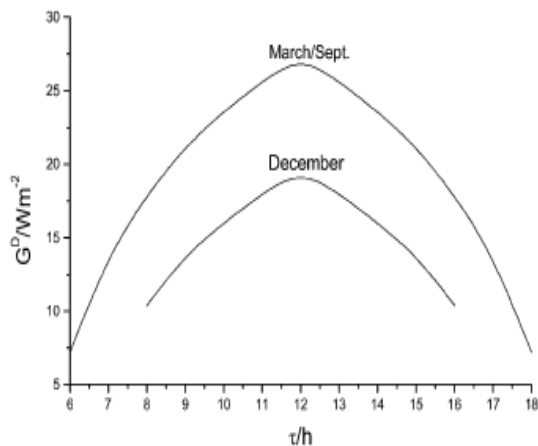
Figure12. Ground irradiance from diffuse (sky) radiation from a clear sky at the shortest winter day and at equinox
