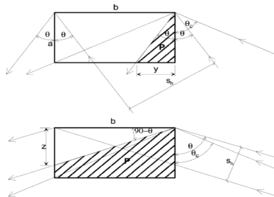
Figure 4. Influence of the azimuth angle \theta \neq 0 on the effectiveness of exposure of the ground to reflected light.
