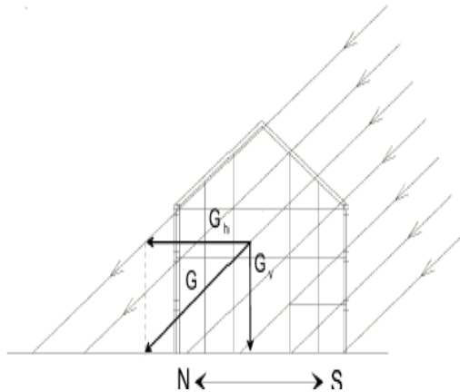
Figure1. Relative horizontal and vertical components of solar radiation
