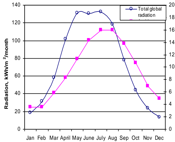
Appendix (1.3). Total global and diffuse radiation
