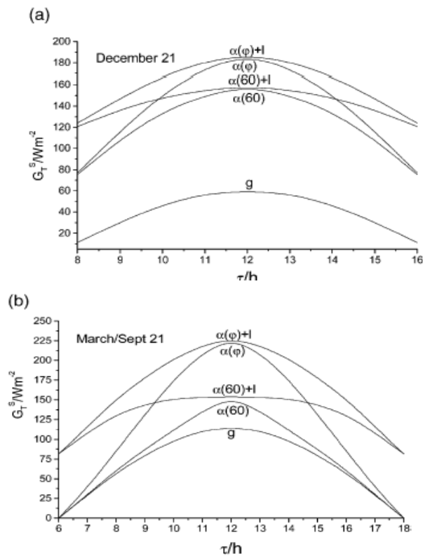
Appendix(1.7). Calculated dependence of ground irradiance on time for the shortest day of the year and for equinox in a greenhouse with a reflecting wall inclined at an angle of 60^\circ , ( \alpha(60) ) with a reflecting wall with variable inclination ( \alpha(\phi) ), without louvers and ( \alpha(60) + 1 ), ( \alpha(\phi) + 1 ) the same but with louvers.
