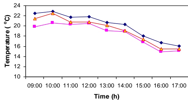
◆ Ambient Temperature ■ Bottom Temperature ▲ Top Temperature ( T_{\text{indoor}} ) ( T_{\text{bottom}} at 50 cm) ( T_{\text{top}} at 150 cm).
