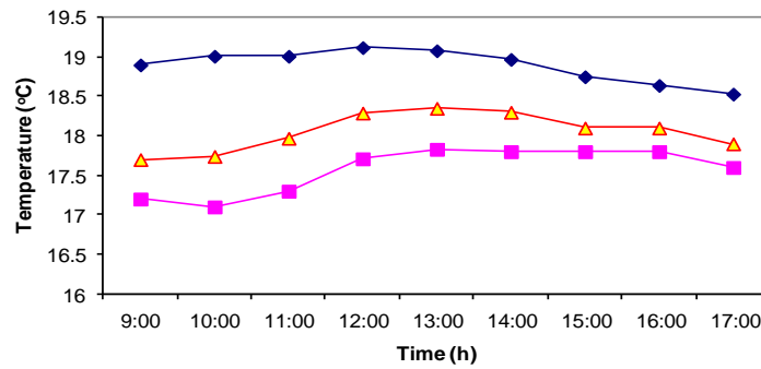
◆ Ambient Temperature ■ Bottom Temperature ▲ Top Temperature ( T_{\text{indoor}} ) ( T_{\text{bottom}} at 50 cm) ( T_{\text{top}} at 150 cm)
