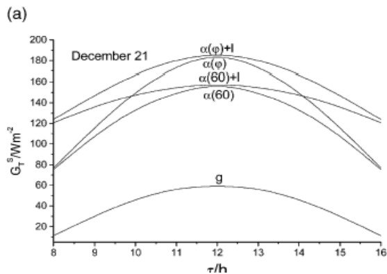
Figure 9. Calculated dependence of ground irradiance on time for the shortest day of the year and for equinox in a greenhouse with a reflecting wall inclined at an angle of 60^\circ , ((\alpha(60))) with a reflecting wall with variable inclination ((\alpha(\varphi)) , without louvers and ((\alpha(60) + 1) , ((\alpha(\varphi) + 1) the same but with louvers.
