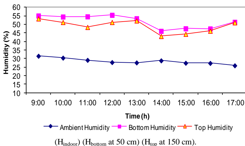
Appendix 2.20. Average daily variation of humidity in November
