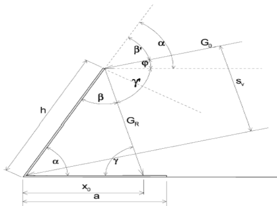
Figure 3. Schematic representation of the reflection of a sunbeam to the ground of a greenhouse with a reflecting wall
