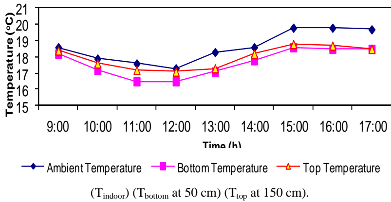
Appendix 2.9. Temperature variation in June
