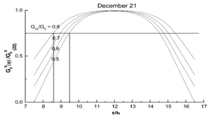
Appendix(1.6). Calculated values of normal irradiance by solar rays relative to the values obtained at the apex on December 21 for different transmittance by the atmosphere.
