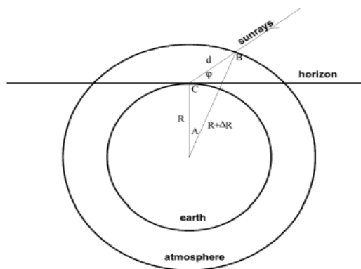
Figure 6. A schematic representation of the earth and its atmosphere with sunrays falling at an inclination \varphi with respect to the horizon
