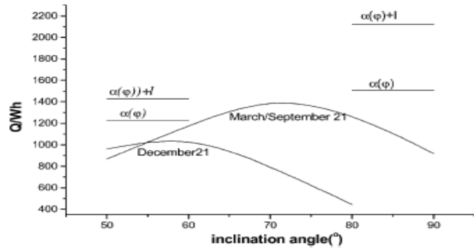
Appendix(1.9). Dependence of the daily energy gain in different types of greenhouses. Different types illustrate the effects of the inclination angle of the wall at the shortest winter day and at equinox. The horizontal lines show the effects of different inclination angles without and with louvers .
