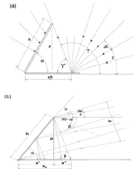
Figure 5. Schematic representations of (a) diffuse light falling onto a point at distance x/h from the reflecting wall, and of (b) diffuse light reflected by the wall.
