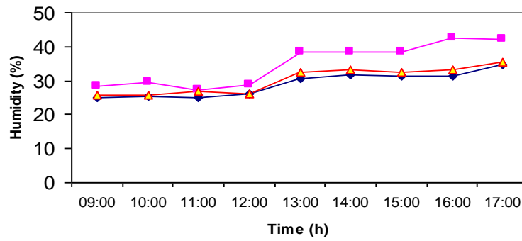
◆ Ambient Humidity ■ Bottom Humidity ▲ Top Humidity ( H_{\text{indoor}} ) ( H_{\text{bottom}} at 50 cm) ( H_{\text{top}} at 150 cm).
