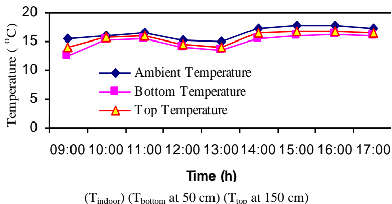
Appendix2.17. Temperature variation in October
