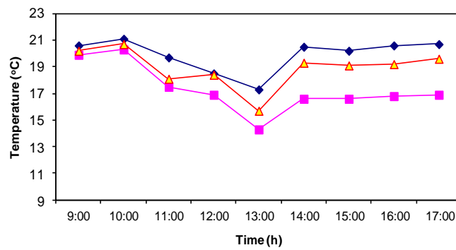
◆ Ambient Temperature ■ Bottom Temperature ▲ Top Temperature ( T_{\text{indoor}} ) ( T_{\text{bottom}} at 50 cm) ( T_{\text{top}} at 150 cm).
