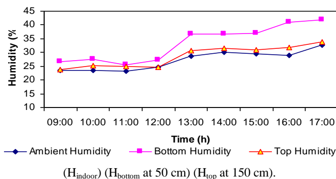
Appendix 5.22. Average daily variation of humidity in December
