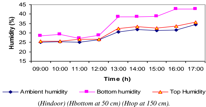
Appendix2.2. Average daily variation of humidity in January
