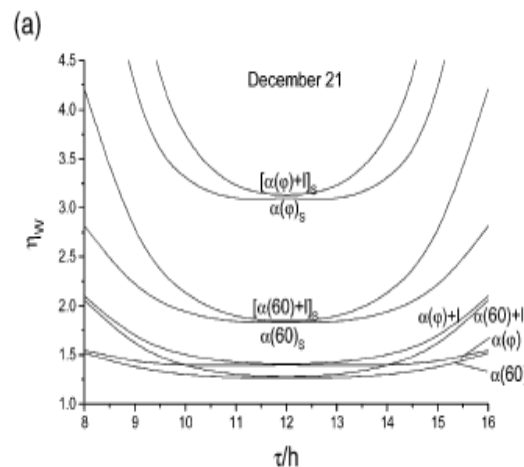
Figure 10. Dependence of the irradiance enhancement coefficient on time, the shortest day of the year and equinox at 44^\circ NL in a greenhouse with reflecting walls inclined at optimum angles \alpha(60) and \alpha(70) , and with reflecting walls with variable inclinations.
