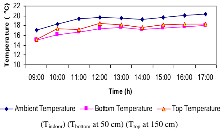
Appendix 2.11. Temperature variation in July
