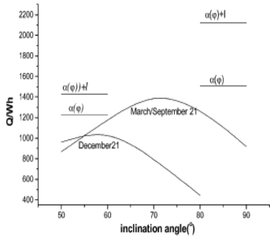
Figure11. Dependence of the daily energy gain in different types of greenhouses. Different types illustrate the effects of the inclination angle of the wall at the shortest winter day and at equinox. The horizontal lines show the effects of different inclination angles without and with louvers.
