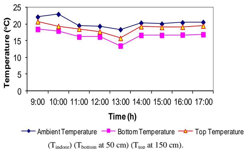
Appendix 2.21. Temperature variation in December
