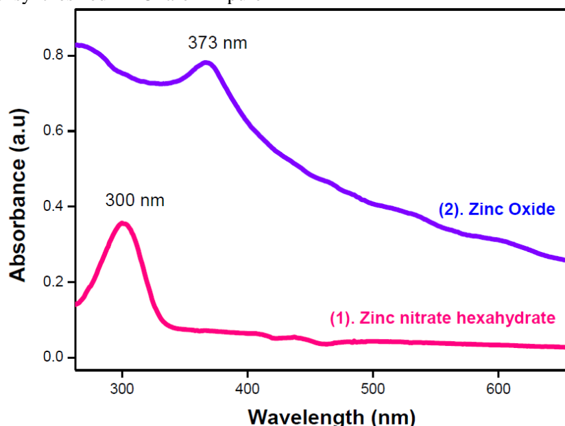
Fig3. UV Spectra of synthesized ZnO nanoparticles
