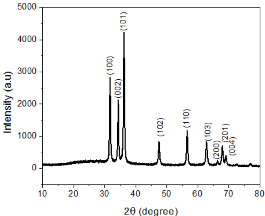
Fig1. XRD pattern of synthesized ZnO nanoparticles
