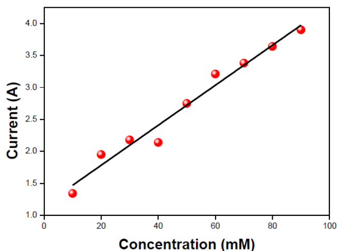
Fig6. Calibration plot
