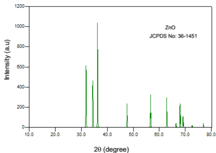
Fig2. XRD pattern of ZnO nanoparticles (JCPDS:36-1451)
