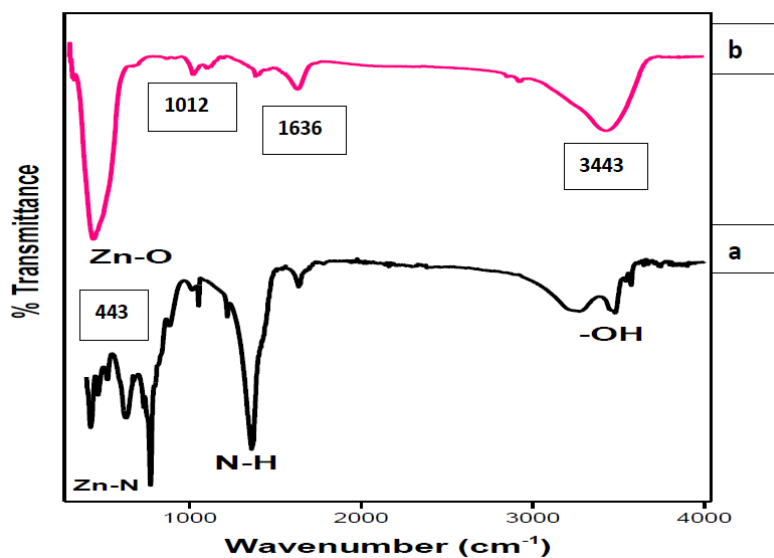
Fig4. (a) FTIR spectra of Zinc nitrate (b) FTIR spectra of synthesized ZnO nano particles
